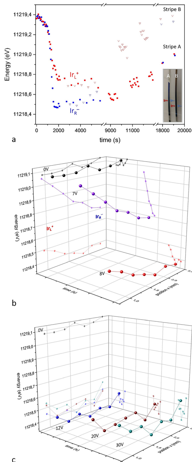
Fig. 11 (a) X-ray absorption energies for the Ir LIII peak during bipolar electrochemistry treatment (5 V first 10 000 seconds) and relaxation after switched off. Induced cathode shown in blue, and induced anode in red. (b) Absorption maxima for Ir LIII signal in XAS across the main axis of the bipolar immersed IrOx in operando conditions, for two spans of external applied voltages. The main process at IrOx occurs at 7 V imposed external voltage, while larger voltages (c) (above 10 V) involve water oxidation and reduction at the induced anode and cathode mostly. Reproduced from ref. 90 with permission from ACS, copyright 2021.
