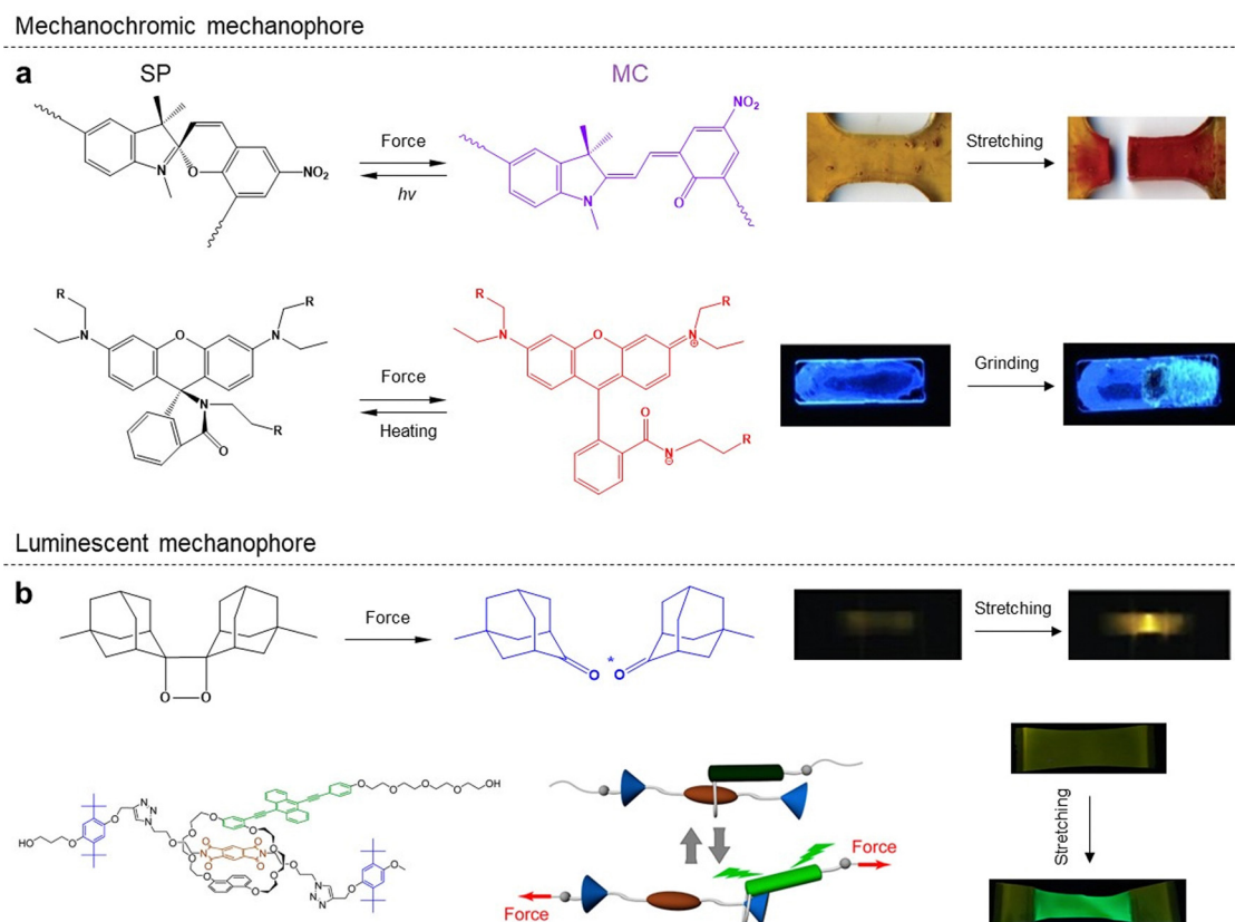
Fig. 4 (a) Under uniaxial extension, spirocyan units were converted into highly colored merocyanine, resulting in a color change in a polymeric material, and chemical structure change of rhodamine-based molecule after grinding, resulting in a blue powder sample; Copyright © 2009, Macmillan Publishers Limited, Copyright © 2013 Wiley-VCH Verlag GmbH & Co. KGaA, Weinheim. All rights reserved. (b) A dioxetane luminescent mechanophore is activated by force and emits light, and supramolecular mechanophores are prepared by locking a fluorophore and quencher in a rotaxane. Copyright © 2012, Springer Nature Limited, Copyright © 2022, American Chemical Society. All rights reserved.
