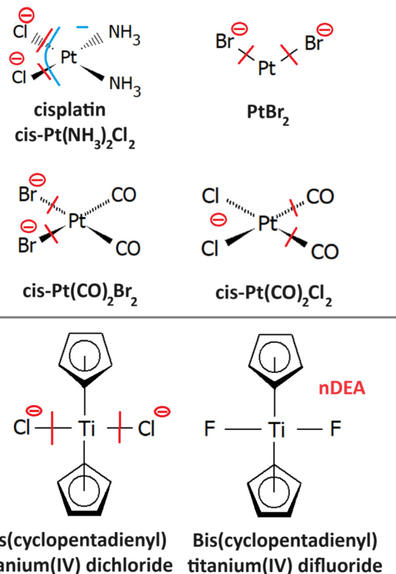
Fig. 10 Radiosensitizers from the group of organometallics and model compounds, whose reactivity with LEEs is discussed in the text: cisplatin (4.1), \text{PtBr}_2 (4.2); \text{PtBr}_2(\text{CO})_2 (4.3); titanocenes (4.4). The red line marks the bond broken in the most intense DEA reaction of the molecule identified for the isolated molecule, and the blue line the dissociation for a solvated molecule. The minus sign marks the anionic DEA fragment.
