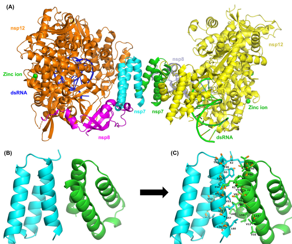
Fig. 1 Structure of the dimeric form of the SARS-CoV-2 RNA-dependent RNA polymerase (RdRp) complex. (A) The cryo-EM structure of the dimeric form of SARS-CoV-2 RdRp in complex with nsp12 : nsp7 : nsp8 : dsRNA and zinc ion is shown, where each subunit is shown as a cartoon in different colours. (B) and (C) The dimeric structure of the nsp7 subunit is shown as a cartoon and the interactions formed by the interface residues are shown and labelled as sticks (with one-letter amino acid codes). The yellow colour dotted line represents the polar contacts between and within the chains.
