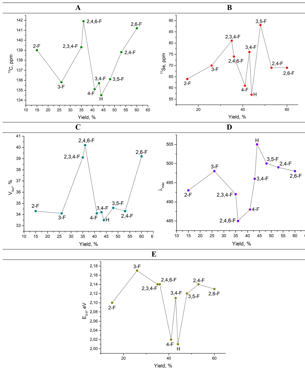
Fig. 6 Effect of the electronic parameters of the NHC F ligand on increasing the hydrothiolation yield. Plot of 13 C (C2) chemical shifts (A). Plot of the 77 Se chemical shift of selenones 5 (B). Plot of the %V bur of 3a-j . (C). Plot of the λ max wavelenghts of Ni/NHC F 4a-g (D). Plot of the E 0-0 energies of Ni/NHC F 4a-g (E).
