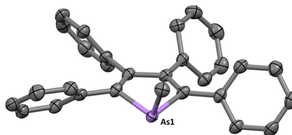
Fig. 5 The molecular structure of \text{MeAsC}_4\text{Ph}_4 ( \mathbf{3} ) in a crystal (50% displacement ellipsoids, phenyl groups simplified and hydrogen atoms omitted for clarity). The As–Me moiety is disordered over two positions and only the major contributor is shown.
