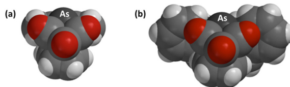
Fig. 4 Corey–Pauling–Kolton models for (a) [\text{Mo}(\text{AsC}_4\text{Me}_4)(\text{CO})_3(\eta^5\text{-C}_5\text{H}_5)] and (b) [\text{Mo}(\text{AsC}_4\text{Ph}_4)(\text{CO})_3(\eta^5\text{-C}_5\text{H}_5)] .
