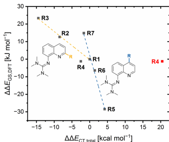
Fig. 6 Plot of the referenced ground state energy differences \Delta\Delta E_{GS,DFT} against the referenced total charge-transfer energy differences \Delta\Delta E_{CT,total} of R1 – R7 (yellow correlation considers R1 and in 2-position alkyl-substituted redox couples, blue correlation considers R1 and in 4-position substituted redox couples, data point of R4 that also considers the O donors is marked red).
