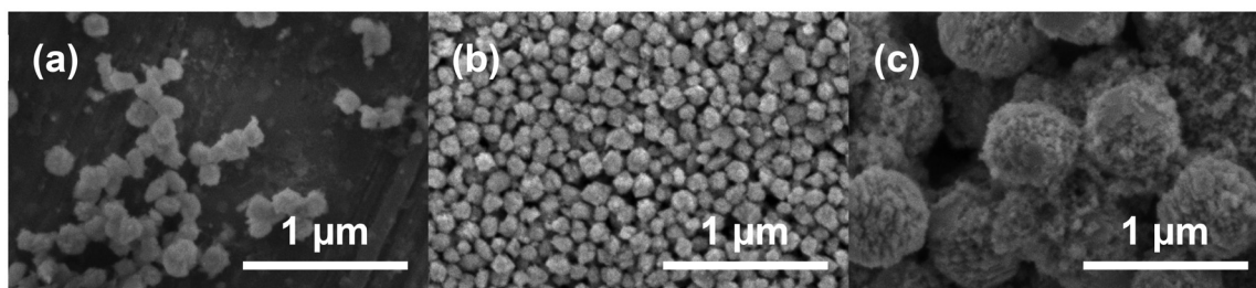
Fig. 7 SEM micrographs of pristine (\text{Zr,U})\text{SiO}_4 solid solutions prepared under hydrothermal conditions ( T = 250 °C, 7 days, pH = 3.0) starting from Zr + U and silicate concentrations of 0.2 \text{ mol L}^{-1} for Zr : U = 80 : 20 (3) (a), 60 : 40 (5) (b) and 40 : 60 (7) (c).
