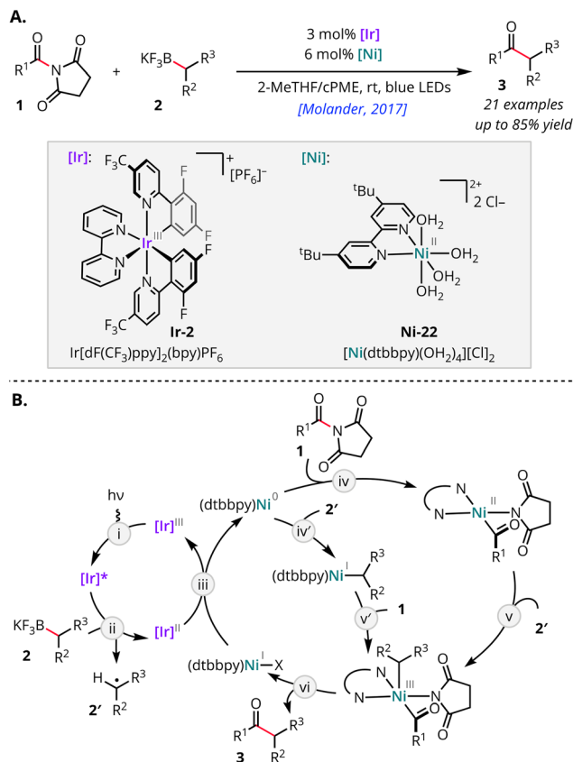
Scheme 15 Key early development in Ni-catalysed acylative coupling using a C(acyl)-N electrophile with dual photoredox and Ni catalysis.
