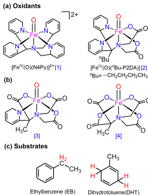
Fig. 2 The investigated (a) [\text{Fe}^{\text{IV}}(\text{O})(\text{N4Py})] (1, left) and [\text{Fe}^{\text{IV}}(\text{O})(^n\text{Bu-P2DA})] (2, right); (b) complexes with sequential replacement of the carboxylate group at the equatorial position; (c) substrates for HAT reactions.
