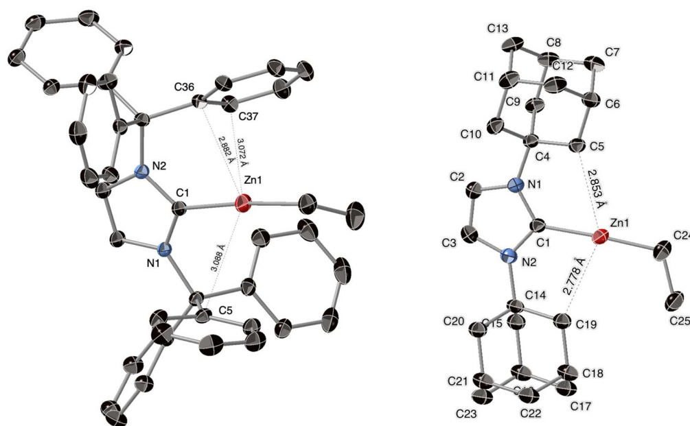
Fig. 3 Molecular structures (ORTEP views) of Zn cations [(ITr)ZnEt] + ([6] + , left) and [(IAd)ZnEt] + ([8] + , right). Selected bond distances (Å) and angles (°). For [6] + : Zn1–C1 = 1.962(1), C1–N1 = 1.353(2), C1–N2 = 1.354(1), Zn1–C42 = 1.930(1), C42–Zn1–C1 = 175.30(6). For [8] + : Zn1–C1 = 1.953(2), C1–N1 = 1.354(2), C1–N2 = 1.359(2), Zn1–C24 = 1.925(2), C24–Zn1–C1 = 176.72(9).
