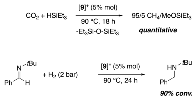
Scheme 4 \text{CO}_2 hydrosilylation and imine hydrogenation catalysis using [9][\text{B}(\text{C}_6\text{F}_5)_4] .
