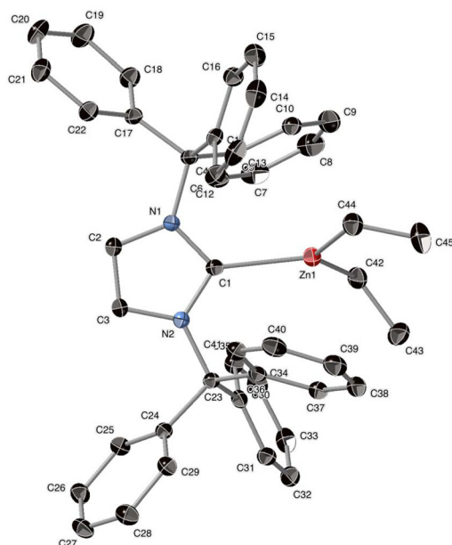
Fig. 2 Molecular structure (ORTEP view) of neutral adduct [(ITr)ZnEt 2 ] ( 2 ). Selected bond distances (Å) and angles (°). Zn1–C1 = 2.154(2), C1–N1 = 1.367(2), C1–N2 = 1.368(2), Zn1–C42 = 2.018(2), Zn1–C44 = 2.012(2), C42–Zn1–C44 = 123.48(8), C44–Zn1–C1 = 116.76(7), C42–Zn1–C1 = 119.74(7).
