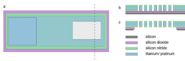
Figure 2 Schematic showing the a) common top-down view, demonstrating exposed contact pad (blue, left) and array (grey, right) area and the cross-sectional view of b) the MNE array and c) MNE array areas (not to scale, number of elements in array illustrative only).
