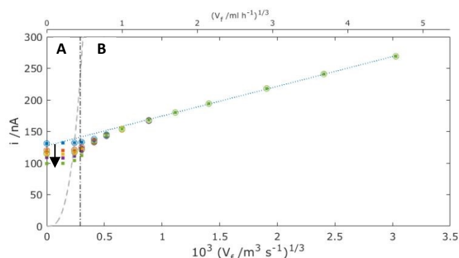
Figure 10 Simulation results for the total MNE array current, i , plotted against V_f^{1/3} for the mass transport limited oxidation of c = 100 \mu\text{M} FcMeOH, at the interelectrode spacing ( p = 120 \mu\text{m} , dots) and without overlap ( p \rightarrow \infty , circles). Data shown are for t = 0.1 (blue), 1 (red), 10 (orange), 30 (purple) and 100 s (green). The dashed line shows the theoretical current which corresponds to the complete oxidation of all the analyte flowing through the pore (Eqn. 4). The dot-dash line shows the calculated flow value from Eqn. 3 where Pe = 1 . The blue dotted line shows the best fit regression line for the region B data above V_f = 1 \text{ ml h}^{-1} .
