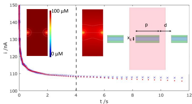
Figure 7 Simulated mass transport limited oxidation current ( x_E = 50 nm, D = 0.70 \times 10^{-9} \text{ m}^2 \text{ s}^{-1} ) for bulk concentration c = 100 \mu\text{M} FcMeOH, for arrays with (red dots) and without (blue crosses) overlap from the diffusion profiles of adjacent electrodes. The dotted line shows the estimated divergence and hence pore diffusion layer overlap time. The insets show the resulting simulated concentration profiles at t = 1 (left – before overlap) and 30 s (middle – confirming overlap), along with (right) a schematic of the simulation region (shaded) showing the pore diameter, d , electrode width, x_E , and edge-to-edge pore spacing, p = 150 \mu\text{m} .
