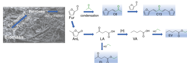
Scheme 1 Catalytic upgrading of biobased furfural to bioproducts with higher number of carbon atoms such as 4-(furan-2-yl)but-3-en-2-one (C8), ethyl levulinate (EL) and ethyl valerate (EV).
