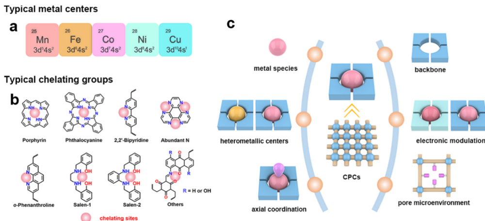
Fig. 3 Design principles of CPCs. (a) Typical metal centers and (b) typical chelating groups of CPCs toward the eCO 2 RR; (c) illustration of the design principle of the CPCs toward the eCO 2 RR.
