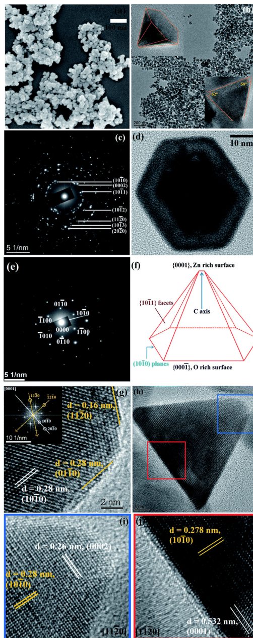
Fig. 6 (a) FESEM image of pure ZnO. (b) Low-resolution TEM image of the pure ZnO nanopyramid. The top-left and bottom-right insets of the figure depict the tilted ( X = 41.1^\circ , Y = 0^\circ ) and side views of a single ZnO hexagonal nanopyramid. (c) SAED pattern of the nanopyramid. (d) A single hexagonal pyramid viewed from the (0001) zone axis. (e) SAED pattern of a single nanocrystal. (f) Schematic presentation of a nanopyramid. (g) HRTEM image of a nanocrystal at the cross-section of two edges of the base. The inset shows the corresponding FFT pattern of the area. (h) Side view of a nanopyramid. (i) HRTEM image of the tip of the pyramid. (j) HRTEM image of the base of the pyramid. Reproduced from ref. 42 with permission from RSC, copyright 2014.
