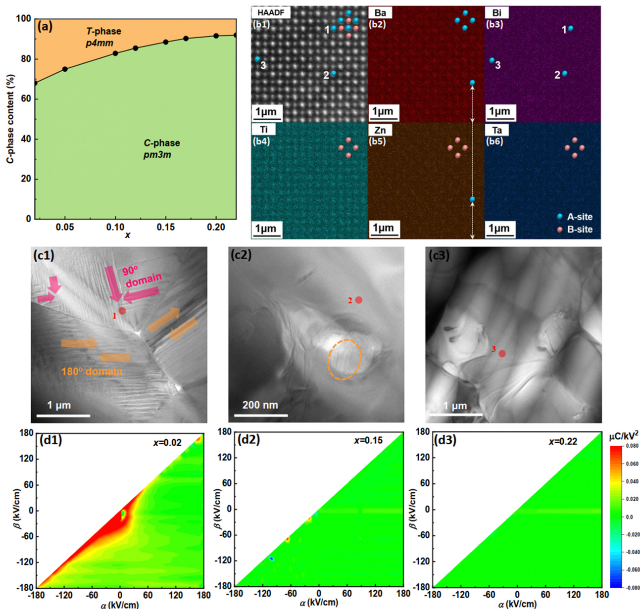
Fig. 1 (a) Phase diagram of BCZT-xBZT with x = 0.02-0.22 ; (b1) HAADF image of BCZT-0.15BZT; (b2)–(b6) atomic-EDS mapping for Ba, Bi, Ti, Zn, and Ta of BCZT-0.15BZT; (c1)–(c3) TEM image; (d1)–(d3) the FORC diagram of BCZT-xBZT with x = 0.02, 0.15 , and 0.22 .
