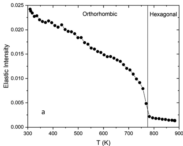
Fig. 7 Elastic intensity as a function of temperature from \text{BaH}_2 measured at BASIS. Reprinted with permission from 334 ( Sci. Rep. , 2022, 12 , 6194).
