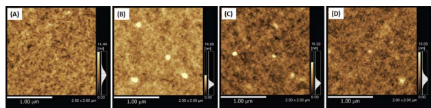
Fig. 18 AFM images of (A) the PEDOS:PSS film, and (B) the B-AuQD-loaded, (C) the G-AuQD-loaded, and (D) the R-AuQD-loaded PEDOT:PSS film. The white spots in (B–D) indicate the domains of aggregated AuQDs. Reproduced from ref. 2 with permission from John Wiley and Sons.
