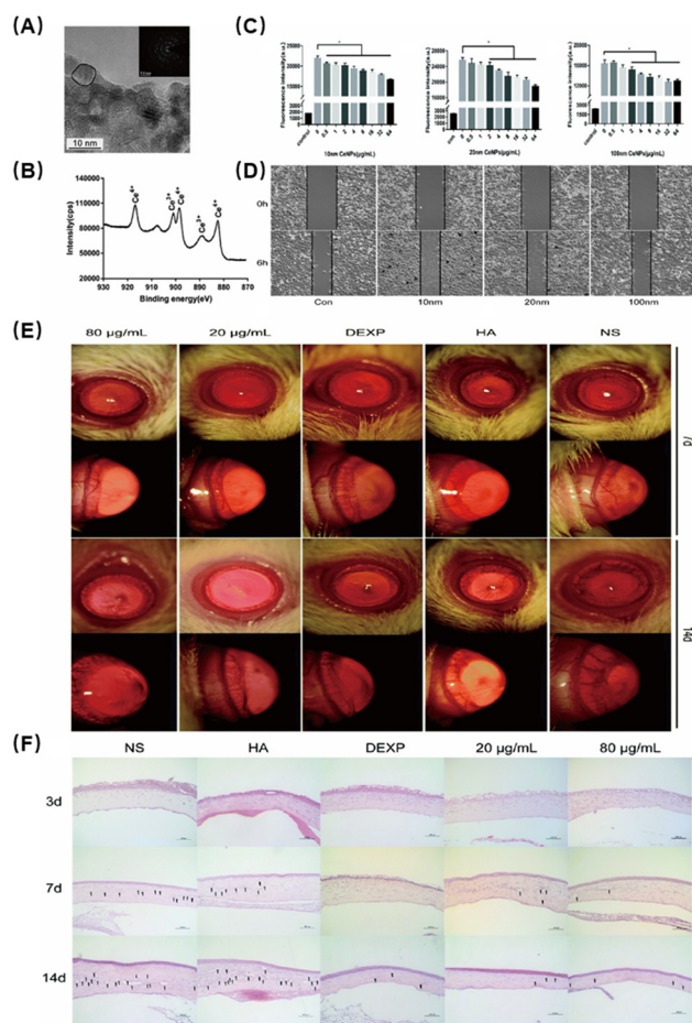
Fig. 6 (A) Representative high-resolution TEM images of CeNPs. (B) X-ray photoelectron spectroscopy spectra of CeNPs. Peaks at 882, 898 and 916 eV are related to Ce 4+ . The peak at 889 eV indicates the presence of Ce 3+ . (C) Effects of oxidized cerium on intracellular oxygen free radicals induced by hydrogen peroxide. Data were analysed using one-way ANOVA, * p > 0.05, n = 3. (D) Migration assays. (E) The inhibitory effect of CeNPs in the corneal neovascularization model. (F) Corneal H&E staining to evaluate the therapeutic effect (200×). Reproduced with permission. 73 Copyright 2019, The Royal Society of Chemistry.
