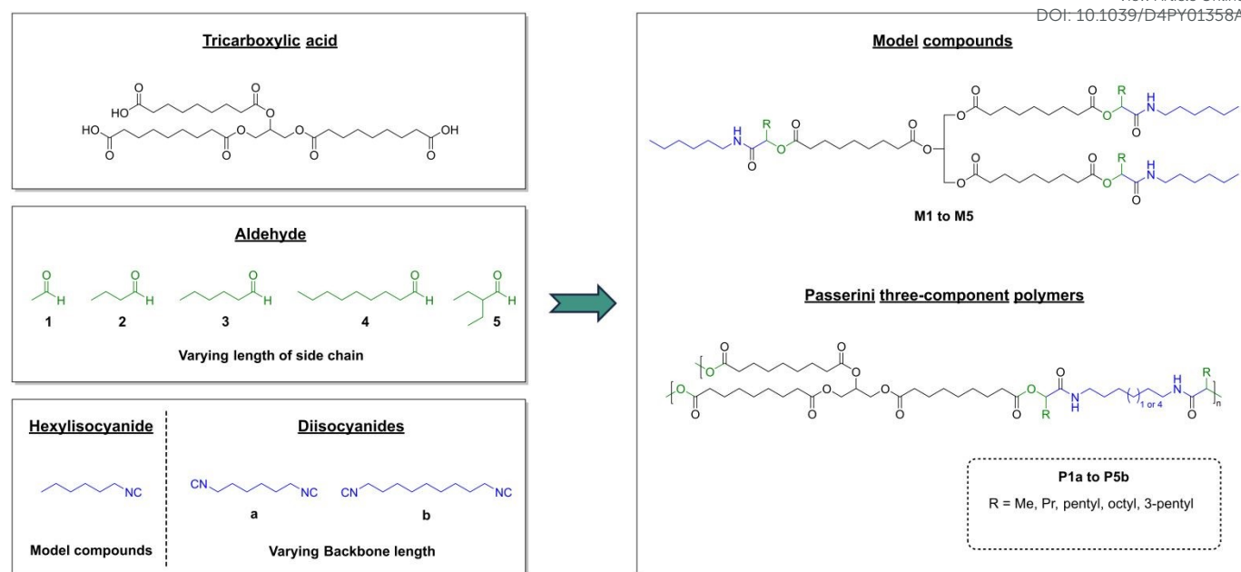
Scheme 2: Synthesis of model compounds M1–M5 (top right) and polymers P1a–P5b (bottom right) via Passerini three-component reaction from the sunflower oil-based tricarboxylic acid, the five aldehydes acetaldehyde ( 1 ) butanal ( 2 ), hexanal ( 3 ), nonanal ( 4 ), 2-ethylbutyraldehyde ( 5 ), and the three isocyanides n -hexylisocyanide, 1,6-diisocyanohexane ( a ) and 1,9-diisocyanononane ( b ).
