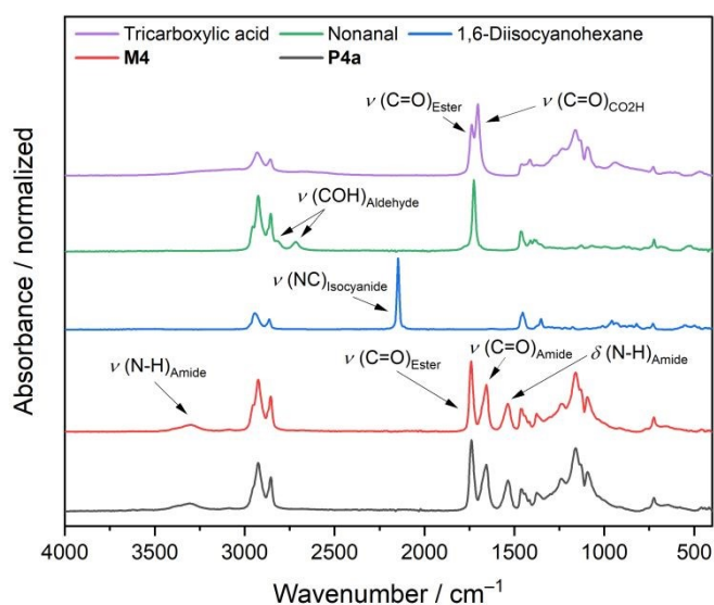
Figure 2: Stacked IR spectra of sunflower oil-based tricarboxylic acid, nonanal ( 4 ), 1,6-diisocyanohexane ( a ), model compound M4 , and polymer P4a . Each IR spectrum is normalized to the strongest absorbance vibration.
