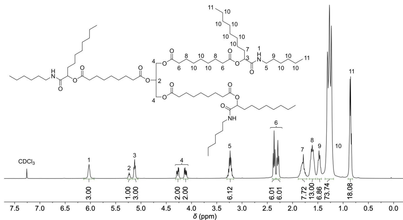
Figure 1: ^1\text{H} NMR spectrum of M4 in \text{CDCl}_3 . Integrals are referenced to protons 4 of the glycerol moiety.
