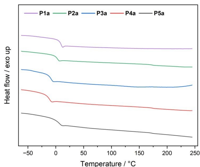
Figure 3: Differential scanning calorimetry measurements of polymers series a .
