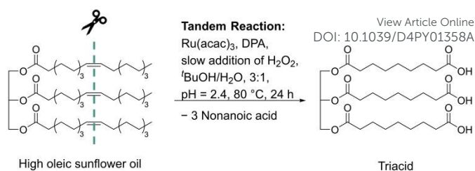
Scheme 1: Ruthenium catalyzed oxidative cleavage of high oleic sunflower oil (DPA: pyridine-2,6-dicarboxylic acid, Ru(acac) 3 : ruthenium(III)acetylacetonate).
