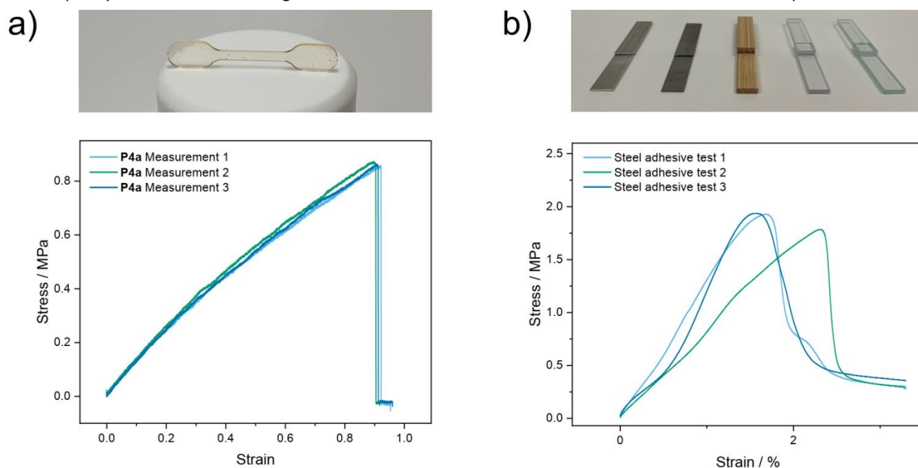
Figure 2: Dog bone sample of polymer P4a with the associated tensile strength measurements (a) and adhesive test samples prepared from polymer P5a and different substrates (aluminum, stainless, wood, PMMA, borosilicate glass) with the adhesive tests of stainless-steel after 2 h of curing at room temperature (b).
