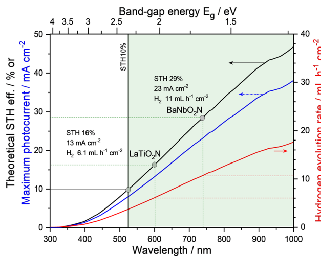
Fig. 4 A graphical representation of the theoretical maximum solar-to-hydrogen (STH) conversion efficiency, maximum photocurrent density, and hydrogen evolution rate as a function of wavelength. Representative perovskite oxynitrides are positioned along the theoretical STH efficiency curve at their respective absorption edges. The three numerical values beside each perovskite oxynitride indicate the efficiency, photocurrent density, and hydrogen evolution rate.
