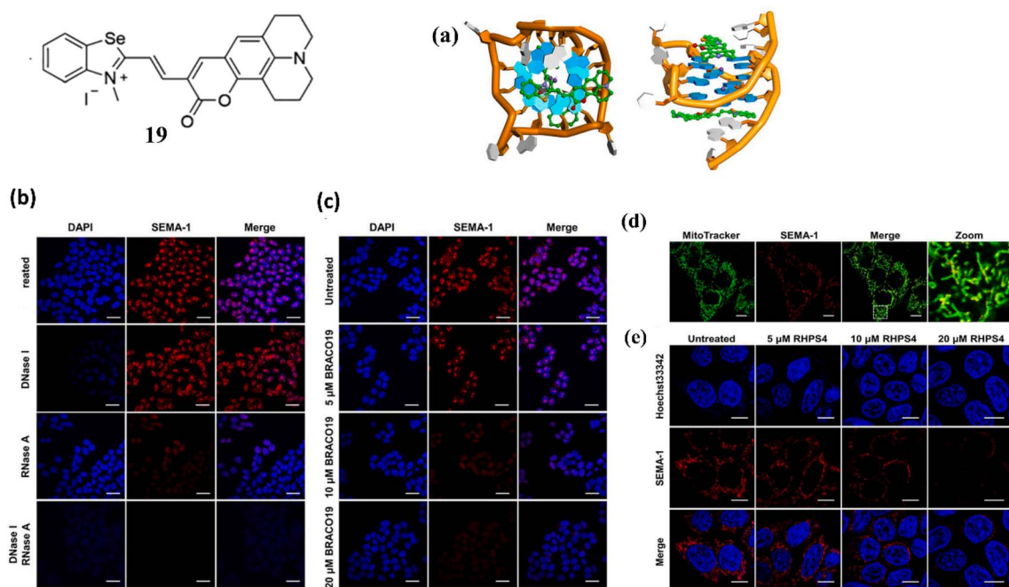
Fig. 15 Structure of ligand 19. (a) Views of the binding mechanisms of 19 with G-quadruplex Pu22 from the top and side. (b) Fixed HeLa cells were stained with 1 \mu M 19 and treated by DNase and RNase. (c) Following the application of 1 \mu M 19 (red) dye, fixed HeLa cells were exposed to varying doses of BRACO19. (d) After being stained with 1 \mu M 19, RHPS4 was applied at varying doses to live HeLa cells (This figure has been adapted from ref. 39 with permission from Elsevier, copyright 2022).
