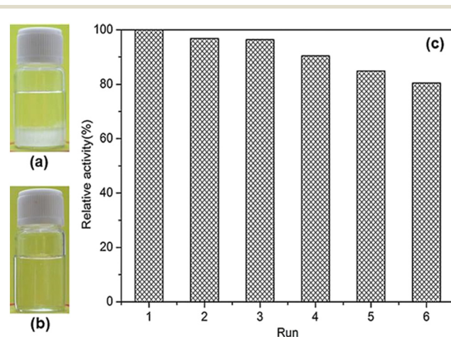
Fig. 19 Photographs of the solutions of the kinetic resolution of ( R,S )- \alpha -methylbenzyl butyrate to ( R )-1-phenylethanol over PAA-PSL at pH 7.0 (a) after cooling to 0 °C and (b) under a new cycle at 55 °C (b). (c) Recycling PAA-PSL in the kinetic resolution of ( R,S )- \alpha -methylbenzyl butyrate to ( R )-1-phenylethanol at 55 °C and pH 7.0. Reprinted with permission from ref. 42, copyright 2018, John Wiley and Sons.
