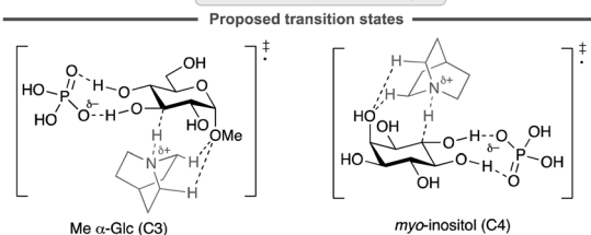
Scheme 51 Site-selective C -alkylations of pyranosides and myo -inositol, and proposed transition state structures for selective HAT. Ir-1 denotes [Ir(dF(CF 3 )ppy) 2 (dtbbpy)]PF 6 ; 4CzIPN denotes 1,2,3,5-tetrakis(carbazol-9-yl)-4,6-dicyanobenzene.
