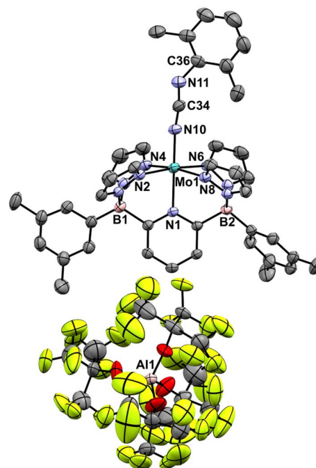
Fig. 6 Molecular structure of [\text{4-Xyl}]^+ . Thermal ellipsoids are shown at the 50% probability level and all H atoms are omitted for clarity. Selected bond distances (Å): Mo(1)–N(1), 2.167(3); Mo(1)–N(10), 1.921(3); N(10)–C(34), 1.210(5); C(34)–N(11), 1.207(5); N(11)–C(36), 1.391(6) selected bond angles (°): N(1)–Mo(1)–N(10), 176.82(12); Mo(1)–N(10)–C(34), 171.8(3); N(10)–C(34)–N(11), 170.1(5); C(34)–N(11)–C(36), 137.1(4).
