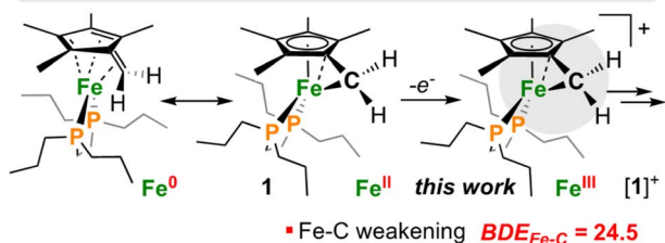
Fig. 1 (A) Overview of intra/intermolecular oxidatively induced reductive elimination with transition metals. (B) Decrease in BDE_{\text{C-C}} in cyclopropane upon oxidation, and this work.
