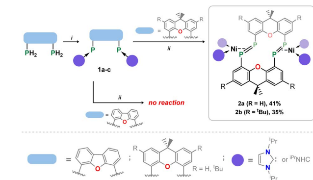
Fig. 2 Molecular structures of (a) 1b , and (b) 2a , with thermal ellipsoids at 30% probability, and hydrogen atoms omitted for clarity. Selected bond lengths (Å) and angles (°) for 1b : P1–C24 1.779(4); P2–C33 1.809(4); C2–P1–C24 106.6(2); C12–P2–C33 96.2(2). For 2a : P1–P2 2.147(1); P1–Ni1 2.260(1); P2–Ni1 2.251(1); P1...P1' 3.542(2); C2–P2–P1 105.3(1); C12–P1–P2 99.0(1); P1–Ni1–P2 56.83(4).
