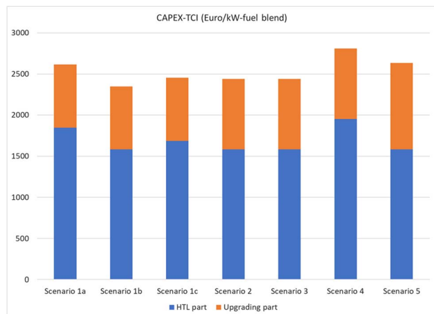
Fig. 14 Summary of CAPEX values for all scenarios.
