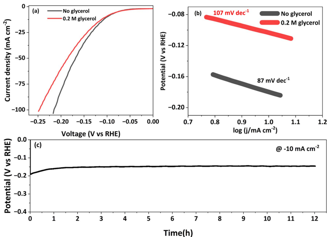
Fig. 6 (a) Cathodic electrocatalytic performances of NCMO/NF for the HER measured through the LSV plots in 1.0 M KOH, and with 0.2 M glycerol. Scan rate employed is 5 \text{ mV s}^{-1} . (b) Tafel plots calculated with NCMO/NF in the presence and absence of glycerol. (c) Twelve-hour sustainability test conducted with NCMO/NF for cathodic HERs at a current density of 10 \text{ mA cm}^{-2} .
