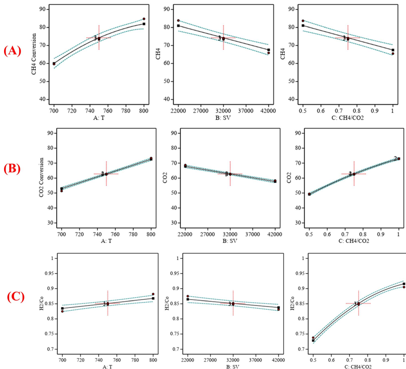
Fig. 6 (A) The relationship between the reaction parameters and \text{CH}_4 conversion percentage; (B) the relationship between the reaction parameters and \text{CO}_2 conversion percentage; (C) the relationship between the reaction parameters and \text{H}_2/\text{CO} ratio.
