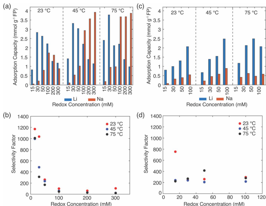
Fig. 3 (a) Uptake of Li + and Na + and (b) \alpha_{\text{Na}}^{\text{Li}} during chemical reduction of FP with redox mediators EDTA-Fe 2+ . (c) Uptake of Li + and Na + and (d) \alpha_{\text{Na}}^{\text{Li}} after reduction by citrate-Fe 2+ . The mediator concentration and reduction temperatures are indicated on the figure. The surrounding brine had a 1 : 78 Li + : Na + molar concentration.
