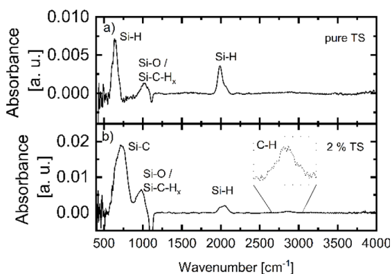
Fig. 7 FTIR spectra of (a) an a-Si:H film deposited at 440 °C with 20 \mu\text{l} trisilane for 10 minutes and (b) an a-Si:H film deposited at 555 °C with 440 \mu\text{l} of 2% trisilane diluted in cyclooctane for 10 minutes. The peaks are labeled with the corresponding bonds. In (b) the Si-H bending vibration peak at 640 \text{cm}^{-1} is overlaid by the strong Si-C peak at around 720–780 \text{cm}^{-1} .
