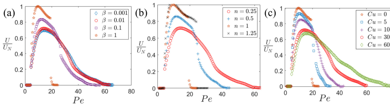
Fig. 7 Variation of normalized axial phoretic velocity of the isotropic colloid with Pe for different values of (a) \beta = (0.001, 0.01, 0.1, 1) for Cu = 30, n = 0.25 , (b) n = (0.25, 0.5, 1, 1.25) for Cu = 30, \beta = 0.01 and (c) Cu = (0, 5, 10, 30, 60) for \beta = 0.01, n = 0.5 . The phoretic axial velocity of the particle in a Newtonian fluid at Pe = 10 ( U_N ) is used for normalization.
