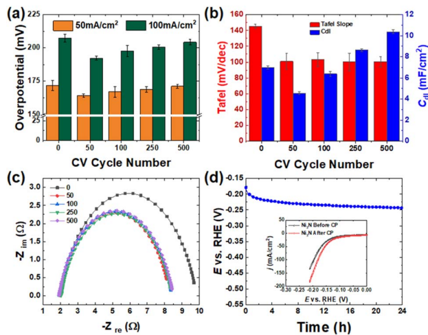
Fig. 7 (a) HER overpotential, (b) C_{dl} and Tafel slope values and (c) Nyquist plots for Ni 3 N/NF before and after anodic CV activation. Note that anodic CV cycle number was changed from 50 to 500 for the activation. (d) 24 h chronopotentiometry of 50 CV-activated Ni 3 N/NF at a constant current density of -20 \text{ mA cm}^{-2} .
