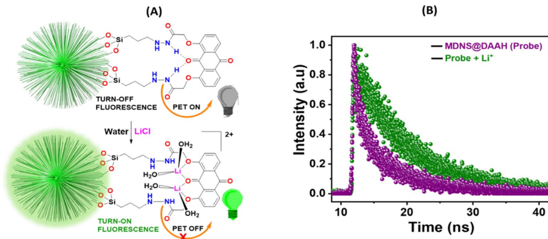
Fig. 8 (A) PET-based turn-on-off mechanism for fluorescence enhancement in MDNS@DAAH with lithium-ion binding. (B) Lifetime measurements of the material MDNS@DAAH before and after the addition of \text{Li}^+ .
