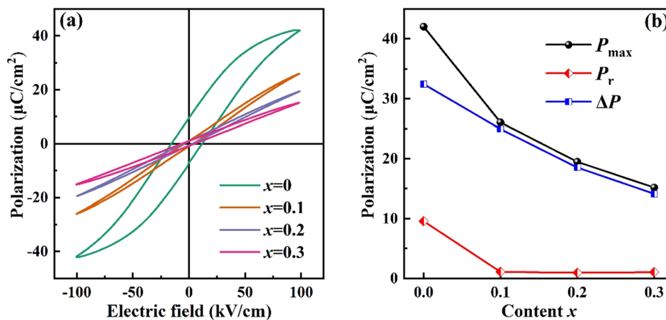
Fig. 5 (a) The bipolar P - E loops at 100 \text{ kV cm}^{-1} of (0.8-x)\text{BNT}-\text{BZT}-x\text{NN} ceramics and (b) P_{\max} , P_r and \Delta P ( P_{\max}-P_r ) as a function of x content.
