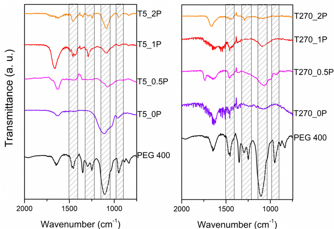
Fig. 4 FTIR spectra of the Bi 19 S 27 I 3 samples compared with PEG 400 for 5 and 270 minutes of reaction. The bands of interest are marked in both graphs.
