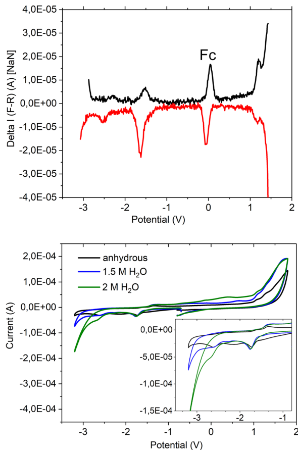
Fig. 5 Electrochemical properties of compound 4a [Pd(PNP-C2-Me)] in anhydrous acetonitrile. Differential pulse voltammogram (voltages referred to ferrocene/ferrocenium, the y-axis shows \Delta Current (A). NaN stands for "not a number", F-R for "forward minus reverse" indicating how the DPV measures its signal) in anhydrous acetonitrile is shown above and cyclic voltammogram including electrochemical traces in the presence of water below: 4a in anhydrous acetonitrile (black), 1.5 M H 2 O in acetonitrile (blue), and 2 M H 2 O in acetonitrile (green). During the study of different amounts of water added, the electrodes were completely stable.
