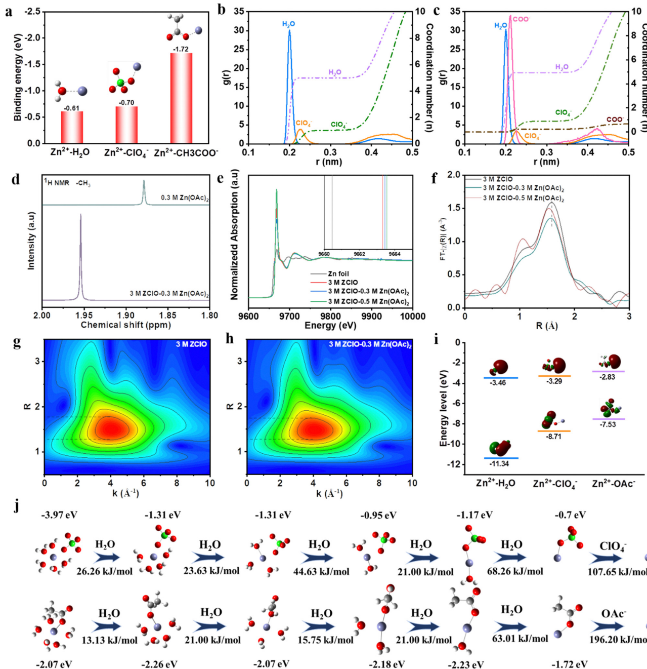
Fig. 2 Investigation of competitive coordination of Zn 2+ . (a) Binding energy of Zn 2+ with different species. (b) and (c) MD results of 3.0 M ZClO electrolyte (b) and 3.0 M ZClO – 0.3 M Zn(OAc) 2 additive (c). (d) 1 H NMR of different electrolytes. (e) Zn K-edge XANES spectra of different electrolytes. (f) Fourier transform EXAFS curves of ZClO electrolyte with various concentrations of additive. (g) and (h) WT-EXAFS of 3.0 M ZClO (g) and 3.0 M ZClO – 0.3 M Zn(OAc) 2 (h). (i) HOMO–LUMO energy levels of various groups. (j) Step-by-step desolvation process of hydrated zinc ions calculated by Gaussian.
