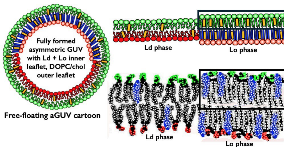
Fig. 11, Left, schematic of an aGUV. Upper right image illustrates the two compositionally different leaflets, with cholesterol as yellow rectangles. This outer leaflet was formed from an SLB of DOPC/cholesterol = 80/20 and includes the green fluorescent dye, TopFluor-PC. Lower right image, the phospholipids and cholesterol shown as more realistic molecular models. The thermodynamically stable Lo and Ld phases are indicated, and the induced order domains are enclosed by black rectangles 23 . Modified from Fig. 2 of 23 .
