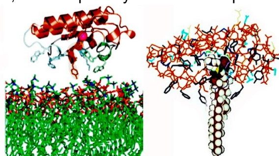
Figure 9, PLA2 and its target lipid, modified from Figs.4&5 of Dennis et al Chem.Rev. 111 . (A) Water-soluble PLA2 penetrates exoplasmic monolayer to bind its PC substrate; (B) 2-chain PC with sn-2 acyl linkage in active site of PLA2. enzyme 33-37 . Surrounding bilayer not shown.
