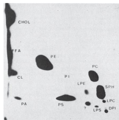
Fig. 3, 2D TLC of MeOH then CHCl 3 extraction of red blood cell lipids showing each phospholipid. Originally 18 Fig.3 of Roelefsen & Zwaal 1976. By phosphate assay of each scraped spot 17 , quantitation is achieved.
