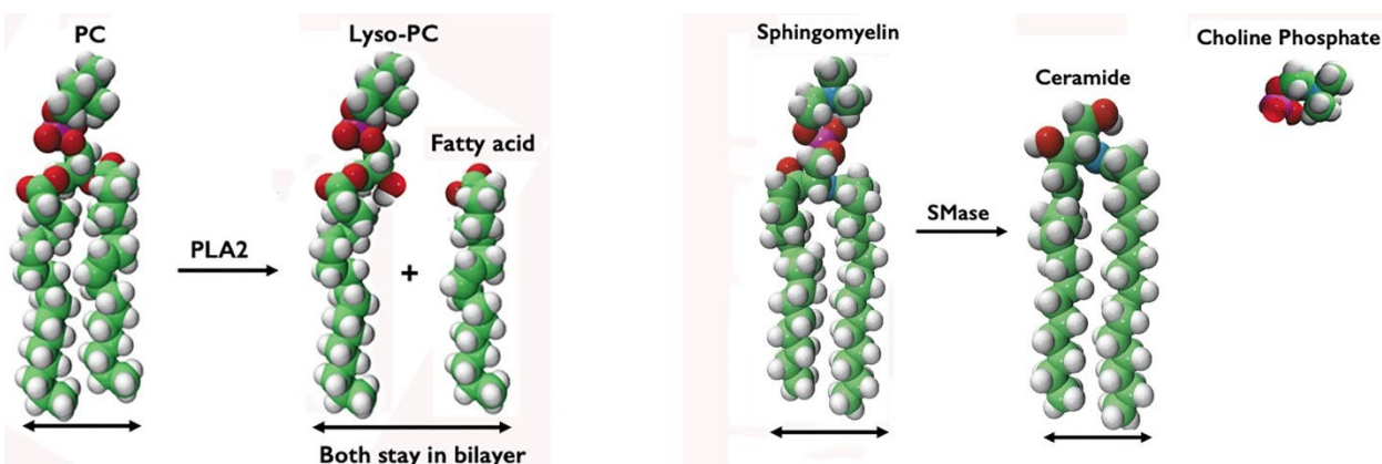
Fig. 8 uses illustrations of molecular models (from Avanti Polar Lipids website) to show that PLA2-catalyzed hydrolysis reaction of PC increases monolayer pressure with both products remaining in the bilayer, whereas SMase enzymatic reaction decreases monolayer pressure, with choline phosphate, soluble in water, leaving the monolayer, and product ceramide 32 being a more condensed lipid than is SM. Double headed arrows give approximate relative indication of lipid area.
