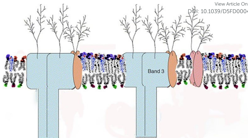
Fig. 7, Cartoon of asymmetric rbc plasma membrane, showing phospholipids to be mostly PC and SM (orange and blue) in the exoplasmic leaflet, and mostly PE and PS (red and green) in the cytoplasmic leaflet.
