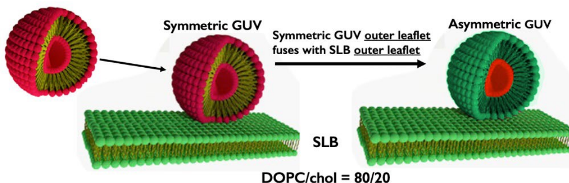
Fig. 10, aGUV preparation by use of hemifusion. The symmetric GUV hemifuses with lipids of a supported lipid bilayer. The original GUV inner leaflet is retained, a new aGUV outer leaflet forms with lipids of the SLB composition. From 47 Fig.1.
