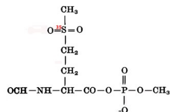
Fig. 4, FMMP = formyl methionyl sulphone methyl phosphate
