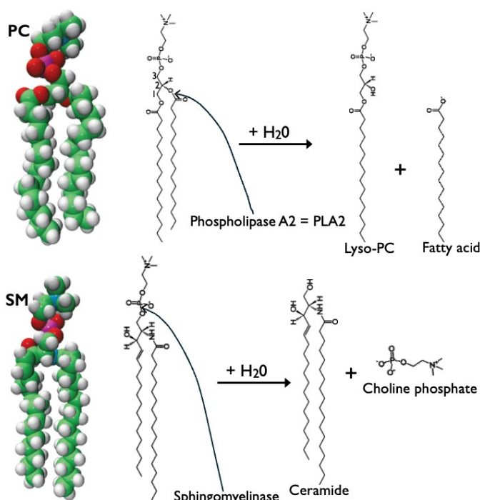
Fig. 6, Specificity of phospholipases A2 and sphingomyelinase, both with central roles in the decade of asymmetry research, 1973-1983. PLA2 and its hydrolysis products lyso-PC and fatty acid remain confined to the exoplasmic leaflet monolayer. SMase and its hydrolysis product ceramide also remain in the exoplasmic leaflet, but product choline phosphate diffuses away into water. Molecular models from Avanti Polar Lipids.
