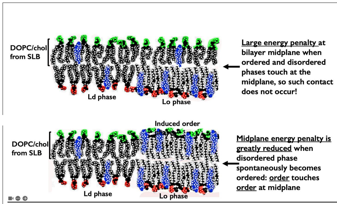
Fig. 13, importance of the asymmetric bilayer midplane area. Upper image shows contact at the bilayer midplane of disordered with ordered phases that would incur a large energy penalty. The lower image shows induced order domains to appear spontaneously to reduce this energy penalty. This would be the same midplane energy penalty that in symmetric GUVs keeps phase-separated domains in their familiar perfect superposition 60 .
