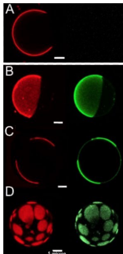
Fig. 12, Fluorescence image data. One symmetric GUV in A, and three examples of induced order B, C, and D. Confocal images show green domains of outer aGUV leaflet to be precisely superimposed on red domains of inner leaflet. (A) Symmetric GUV of DSPC/DOPC/chol having phase-separated Lo + Ld. Image is GUV equator. Red DiD prefers Ld phase, the connecting Lo phase is dark. Lo order is intrinsic thermodynamic order, not induced; (B) Z-stack of aGUV with one large Ld and one large Lo domain. DiD in inner leaflet labels Ld red, leaving Lo dark. TFPC in outer leaflet labels Ld green, leaving induced order domain dark. This induced order domain is entirely DOPC/chol; (C) aGUV equator showing 3 phase domains. Inner leaflet red DiD prefers Ld, leaving Lo dark. Outer leaflet green TFPC prefers Ld, leaving induced order domain dark; (D) Z-stack of aGUV showing many phase domains. DiD in inner leaflet labels Ld red, leaving Lo dark. TFPC in outer leaflet labels Ld green, leaving induced order regions dark. Scale bars show 5 micron. Modified from Fig. 3 and Fig. 5 of 59 .
