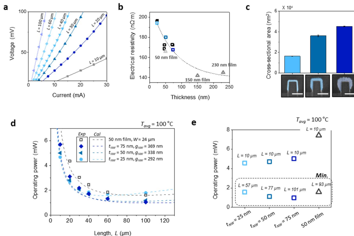
Fig. 4 (a) I - V measurement data for different lengths of nanowires with a thickness of 25\ \text{nm} , as shown in Fig. 3. (b) Electrical resistivity as a function of nanowire and film thickness. (c) Measured cross-sectional areas of nanowires with thicknesses of 25\ \text{nm} , 50\ \text{nm} , and 75\ \text{nm} , along with their corresponding SEM images (measurements from three different nanowires, scale bar = 200\ \text{nm} ). (d) Calculated (dashed line) and measured (dots) operating power required to reach 100\ ^\circ\text{C} for heaters of different lengths, using a 50\ \text{nm} film with a width of 24\ \mu\text{m} as the reference. (e) Operating power extracted from (d) at a length of 10\ \mu\text{m} and at the length with minimum operating power.
