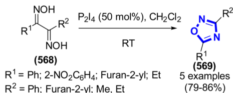
Scheme 151 Synthesis of 1,2,4-oxadiazole derivatives catalyzed by P_2I_4 .
