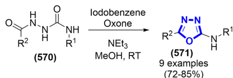
Scheme 152 . Synthesis of oxadiazole moieties catalyzed by NEt 3 .
