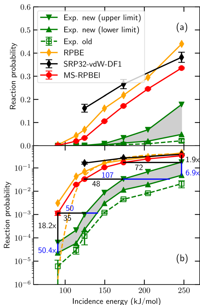
Fig. 1 Sticking probabilities computed 43 for HCl + Au(111) with the MS-RPBE meta -GGA DF, 43 the RPBE GGA DF, 44 and the SRP32-vdW1 DF featuring semi-local exchange and non-local correlation 45 are compared to experimental results, for normal incidence. The open green squares are the experimental sticking probabilities first published, 46 while the upper base and lower base triangles represent upper and lower bounds to the experimental S_0 obtained from an improved analysis of the experiments. 43 Panel (a) uses a linear and panel (b) a logarithmic scale for S_0 . In panel (b) results of QCT 44 (orange diamonds connected by solid orange line) as well as of QD 47 (orange dashed lines) calculations using the RPBE DF are presented. Figure taken from ref. 43 ( https://doi.org/10.1021/acs.jpcc.0c03756 ). Further permission requests to be directed to the ACS.
