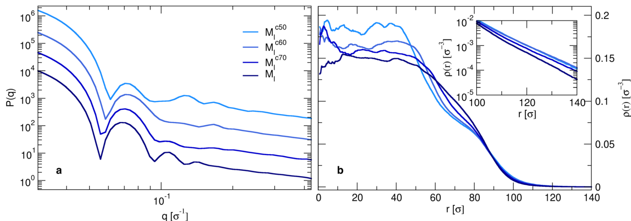
Fig. 5 (a) Numerical form factors P(q) as a function of the wavenumber q and (b) corresponding radial density profiles as a function of the distance r for the M_1^{c50} , M_1^{c60} , M_1^{c70} and M_1 in silico microgels. Inset: Zoom on the long distance tail of the radial density profile.
