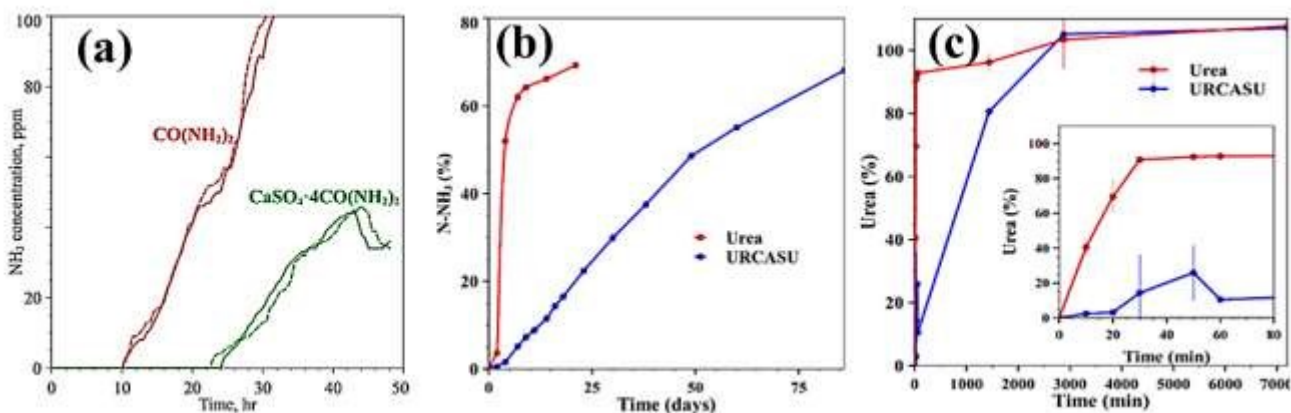
Figure 6. (a) \text{NH}_3 emissions from urea and \text{CaSO}_4 \cdot 4\text{urea} (abbreviated as URCASU) until 50 hours from (38) which was measured in silt loam soil. The measurements were taken over 48 hours under static conditions, with the chamber maintained at 23^\circ\text{C} and a relative humidity level of 50–60% (38). (b) \text{NH}_3 emissions from the same compounds according to the work (43) but until 75 days. The measurement was done in soil, either urea or \text{CaSO}_4 \cdot 4\text{urea} , which was added to a flask containing a thick layer of soil. The relative humidity was approximately 90% and the \text{NH}_3 released was consistently captured in a 0.2\text{ N H}_2\text{SO}_4 solution and quantified using a methyl red indicator. Moreover, mini prills of urea served as the reference, while the urea cocrystal prepared mechanochemically was tested in its powdered form. However, the experiment was designed to compare the \text{NH}_3 emissions from these two nitrogen sources under controlled conditions (43). (c) the kinetic dissolution of urea (43). The samples of urea and its cocrystal were formed into pellets using a hydraulic press. For the static dissolution test, a single pellet was placed in an Erlenmeyer flask containing distilled water and maintained at room temperature for 120 hours. A urea pellet served as the control. Dissolution rates were measured by taking 0.5\text{ mL} samples from the solution at regular intervals (43).
