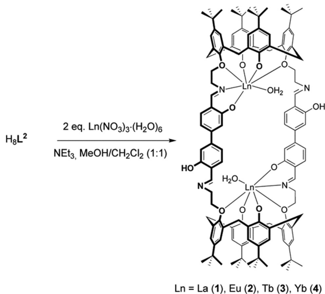
Scheme 2 Synthesis of the complexes [\text{Ln}_2(\text{H}_8\text{L}^2)(\text{H}_2\text{O})_2] (Ln = La (1), Eu (2), Tb (3), Yb (4)).
