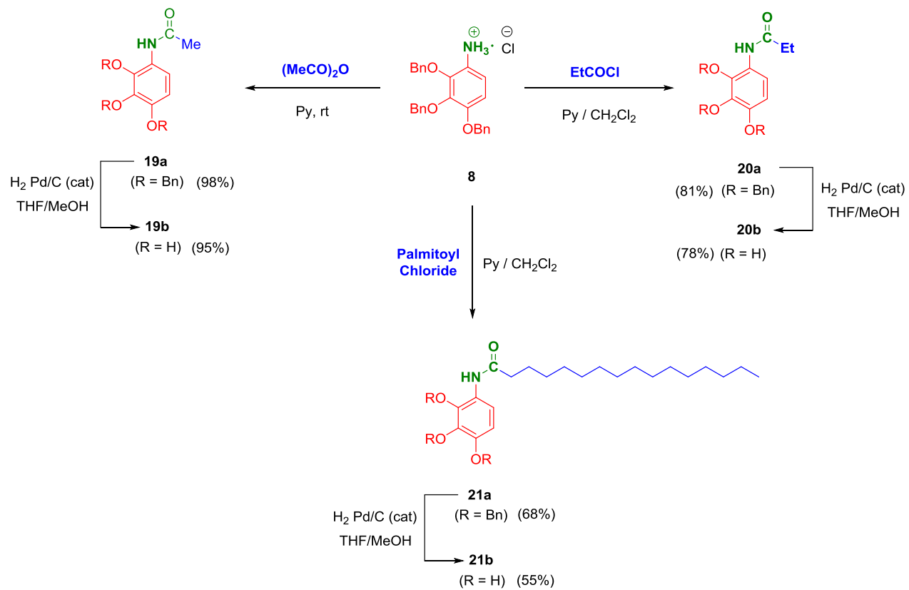
Scheme 5. Synthesis of monopodal amide-linked compounds 19-21 .
