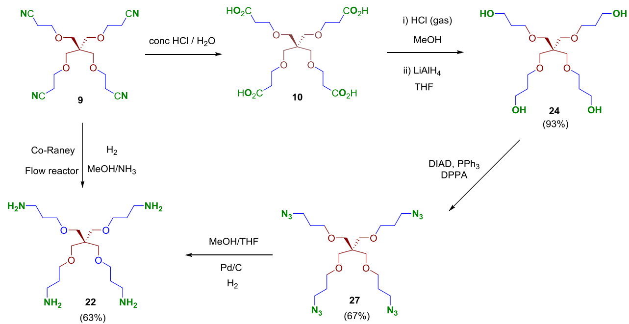
Scheme 8. Synthesis of tetrapodal polyamine ( 22 ) and polyazide ( 27 ) scaffolds.
