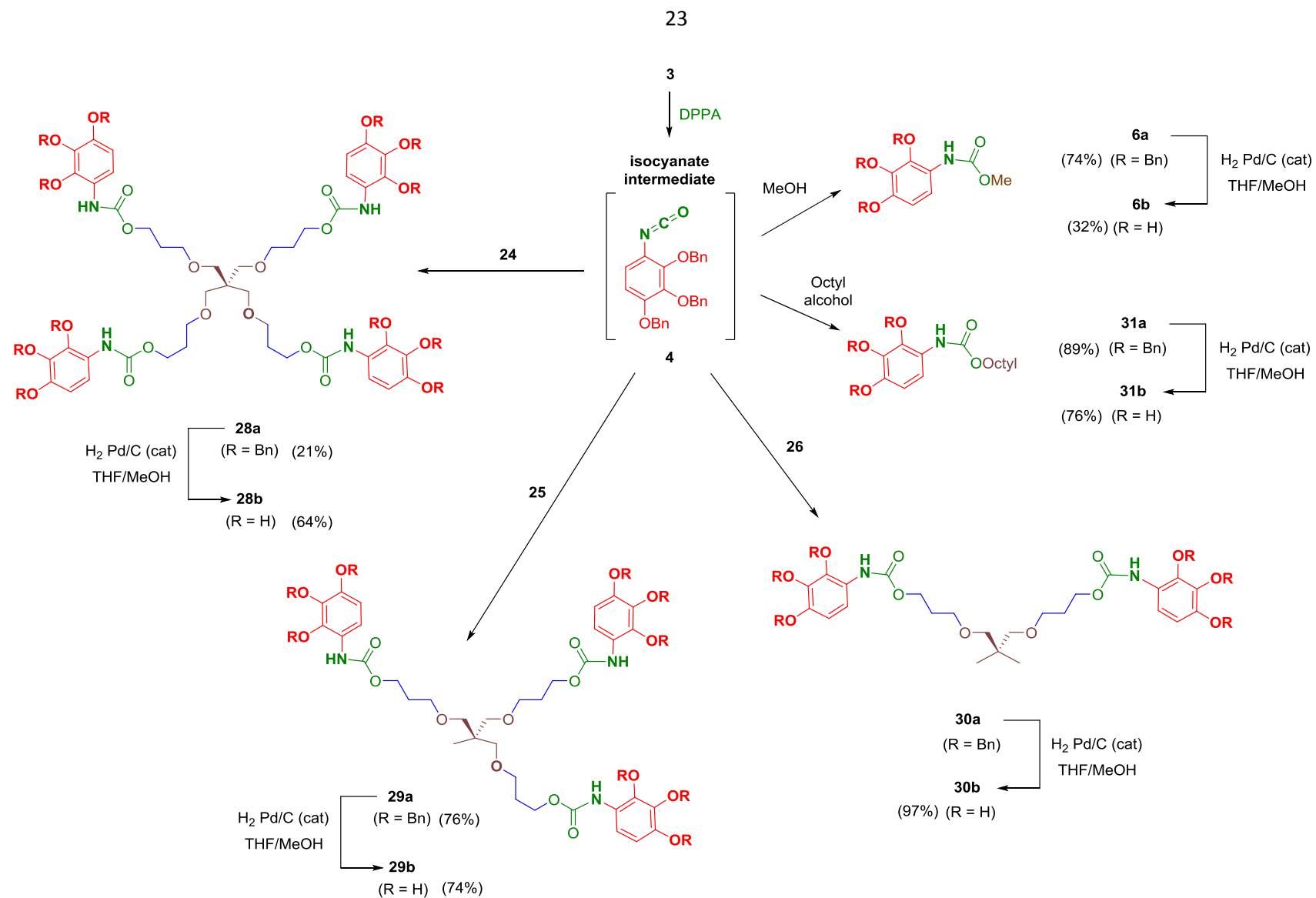
Scheme 9. Synthesis of carbamate-linked series from key isocyanate 4 .
