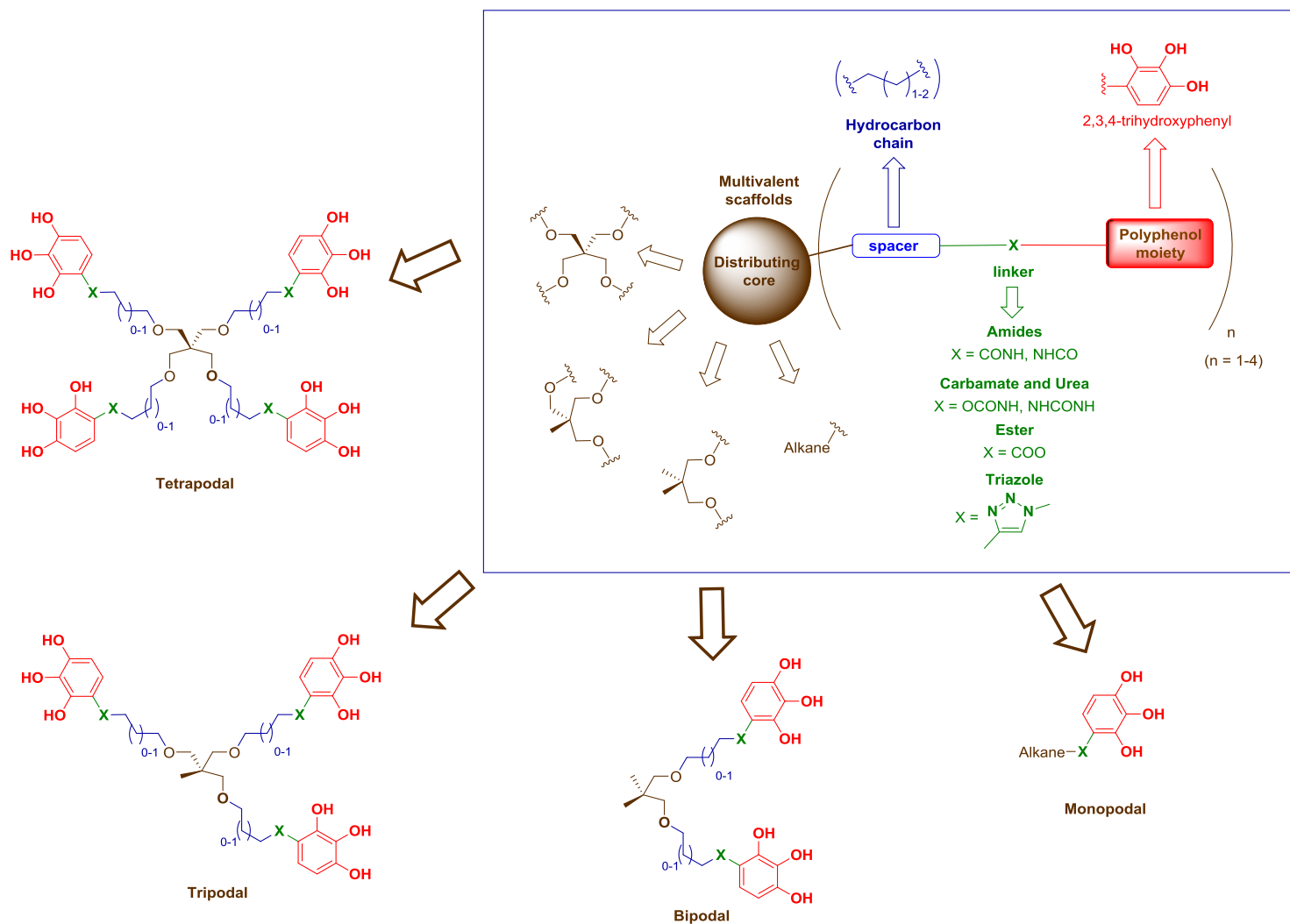
Figure 1. Architecture of the proposed synthetic tannins.
