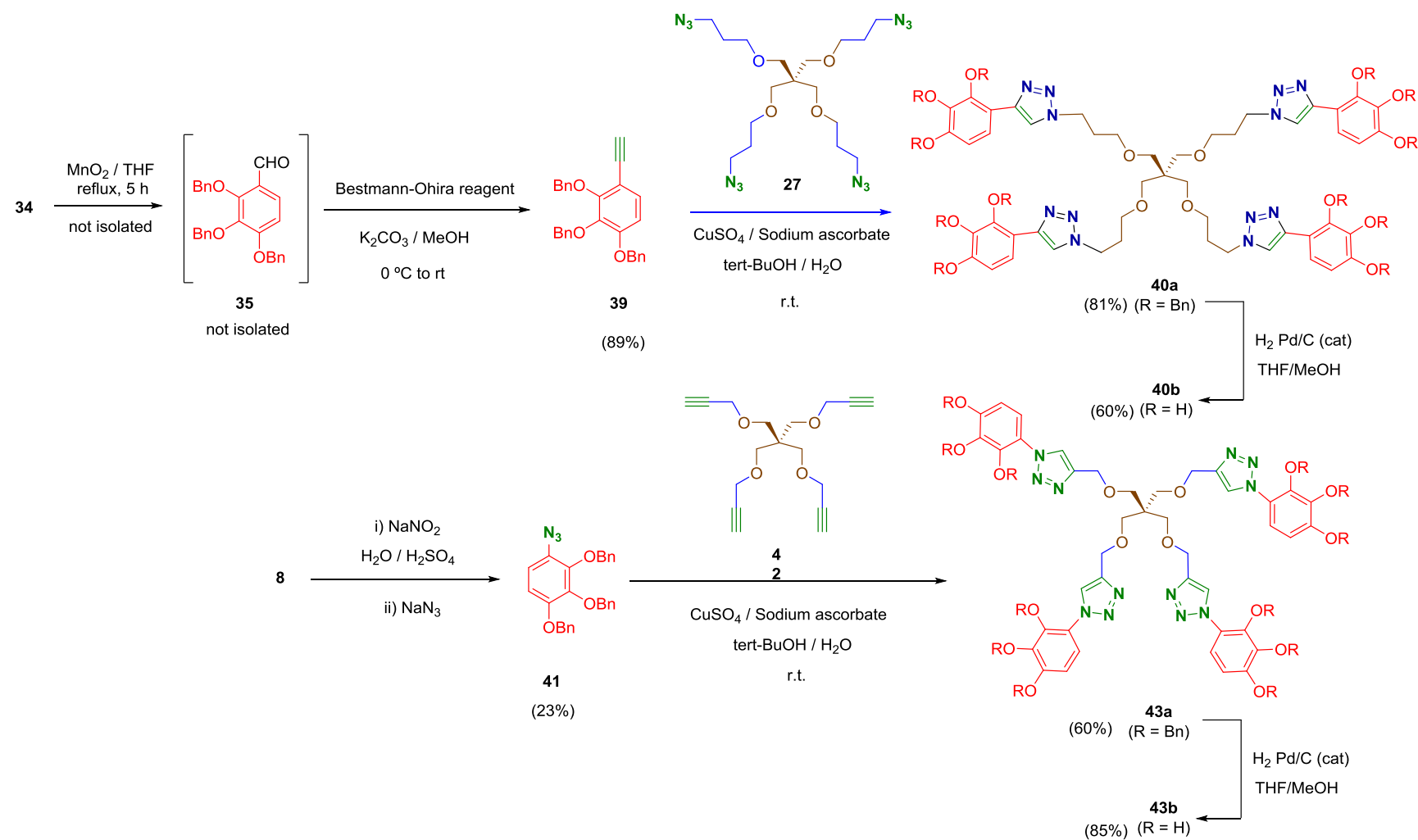
Scheme 12. Synthesis of tetrapodal triazole-linked polyphenols.
