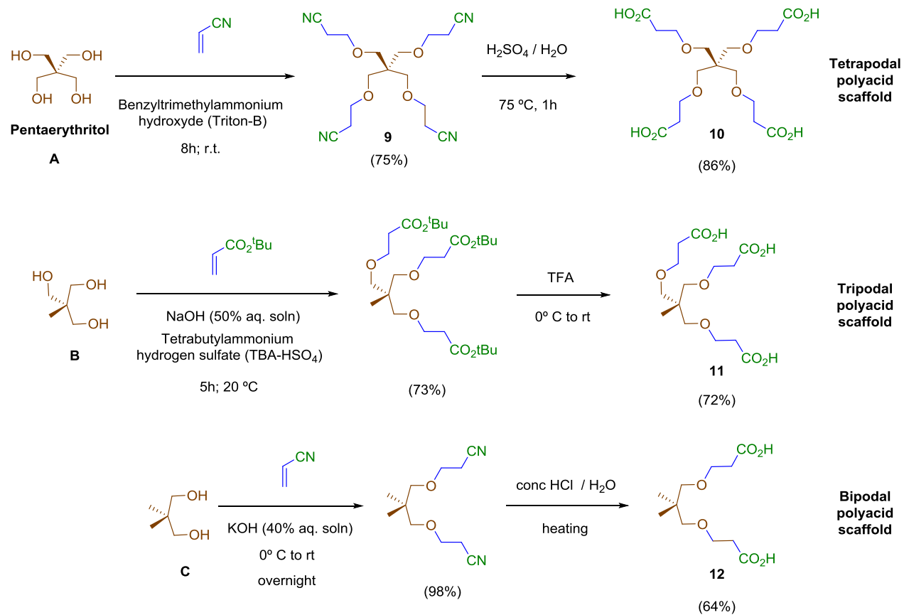
Scheme 2. Synthesis of multipodal polyacid scaffolds 10-12 .
