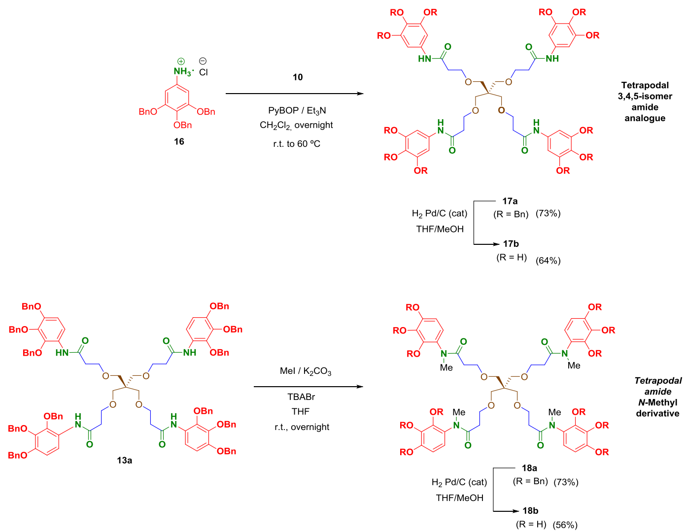
Scheme 4. Synthesis of amide-linked tetrapodal compounds 17-18 .
