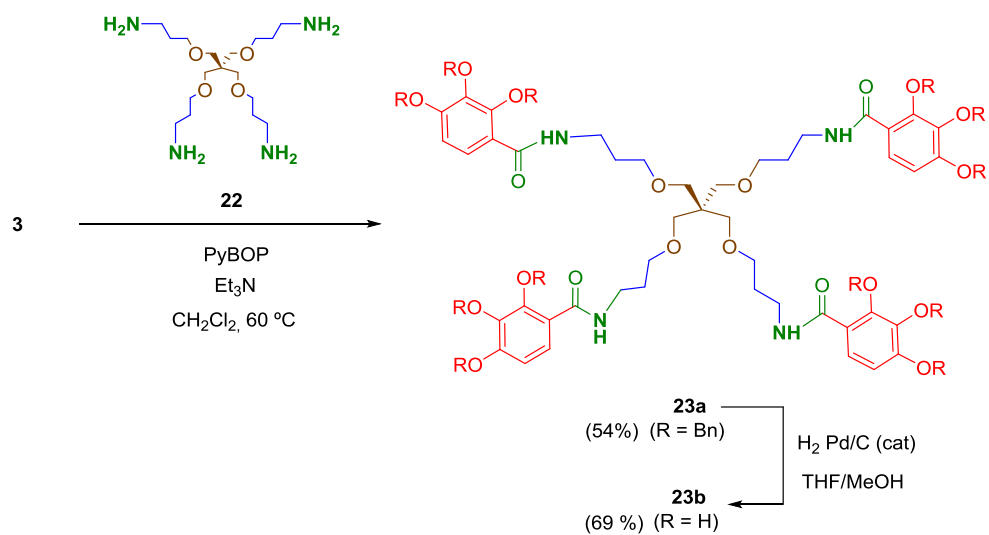
Scheme 6. Synthesis of tetrapodal amide 23b .
