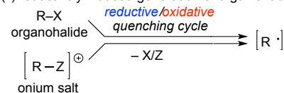
Scheme 3 Generation of various C-centered radicals highlighted in this review.
