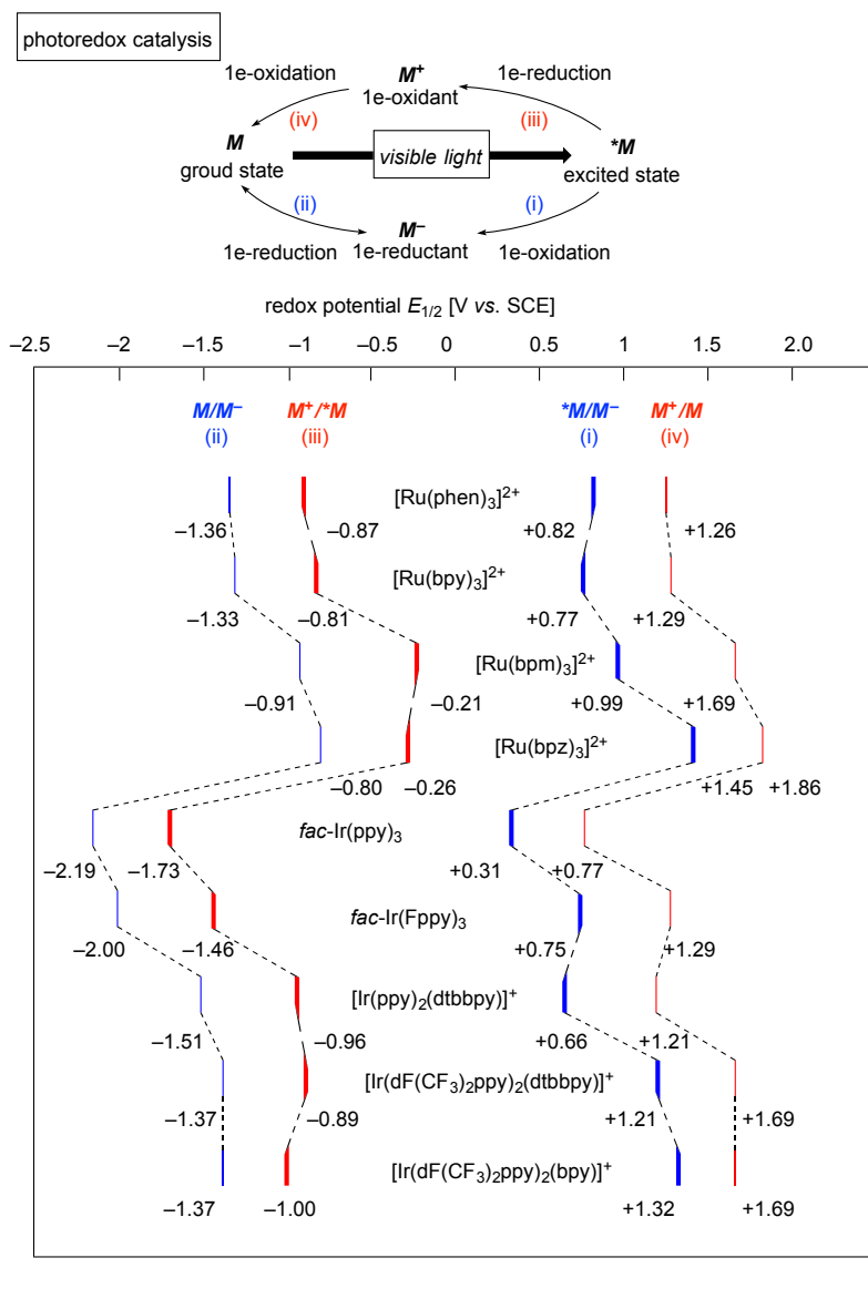
Scheme 2 Photoredox catalysts featured in this review. The redox potentials for ^*[\text{Ir}(\text{Fppy})_3] were calculated based on literature data. 5e,h
