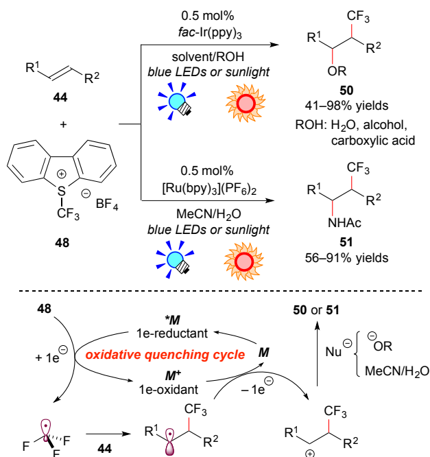
Scheme 23 Photoredox-catalyzed difunctionalization of alkenes through construction of a \text{C}-\text{CF}_3 bond.
