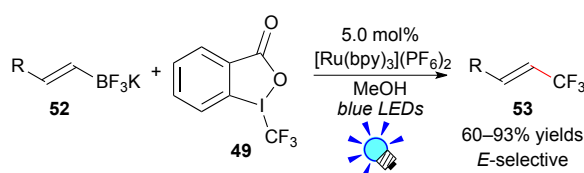
Scheme 24 Photocatalytic synthesis of \text{CF}_3 -alkenes via deboronation.
