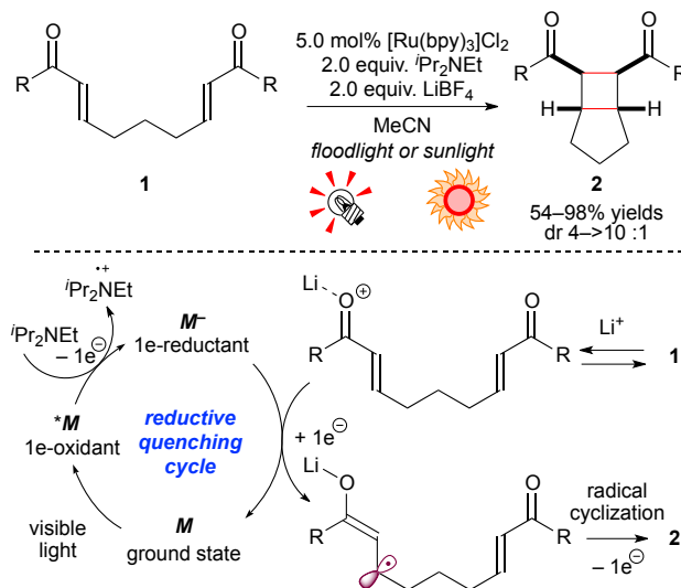
Scheme 4 [2+2] cycloadditions of electron-deficient alkenes through reductive quenching cycle.
