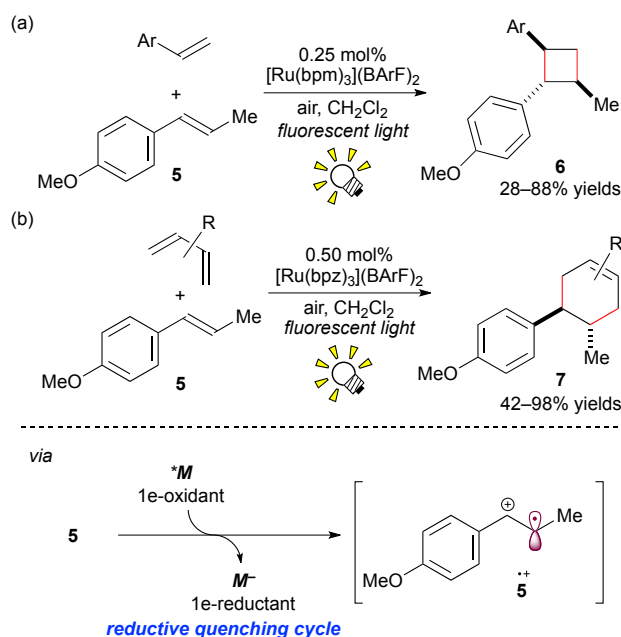
Scheme 6 (a) Crossed intermolecular [2+2] cycloaddition of styrenes (b) Radical cation Diels-Alder cycloadditions.
