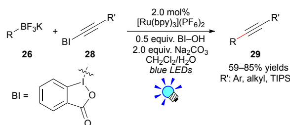
Scheme 13 Photocatalytic deboronative alkynylation.
