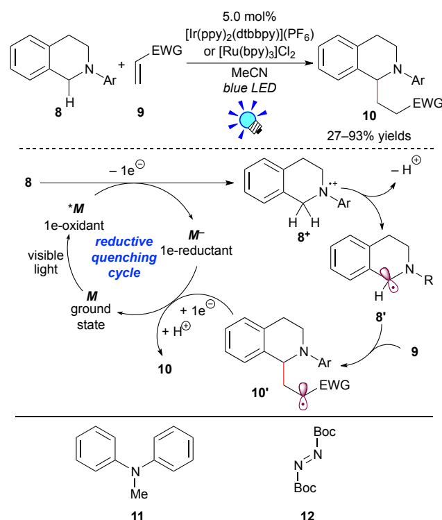
Scheme 7 Addition of \alpha -aminoalkyl radical to electron-deficient double bonds.
