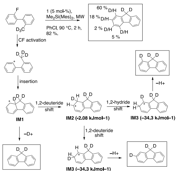
Scheme 4. Deuterium distribution in 3 produced from 2-d 3 ; postulated intermediates and their computed energetics.
