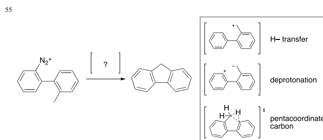
Scheme 3. Postulated mechanisms for the Mascarelli reaction. 10,11,14,15
