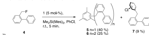
Scheme 6. Product distribution from abstraction of fluoride from 4 .
