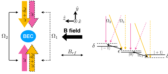
Fig. 1 Three mechanisms including two types of Raman laser coupling ( \Omega_1 and \Omega_2 ) and a rf field coupling ( \Omega_{rf} ) are applied to drive transitions between different hyperfine spin states. The Zeeman level diagram of a ^{87}\text{Rb} atom in a weak magnetic field. The hyperfine state of ^{87}\text{Rb} in the F = 1 manifold is split into three Zeeman levels.
