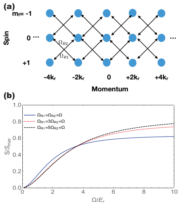
Fig. 6 (a) Creating entanglement between spin and momentum degrees of freedom of a BEC using two types of Raman laser couplings. Type 1 Raman coupling has the selection rule ( \Delta m_f = \pm 1, \Delta p = \mp 1 ). Type 2 Raman coupling has the selection rule ( \Delta m_f = \pm 1, \Delta p = \pm 1 ). (b) The relative entanglement entropy as a function of the coupling strength at zero detuning for both Raman lasers. The dependence of the von Neumann entropy is shown for different ratios of the two Raman coupling strengths.
