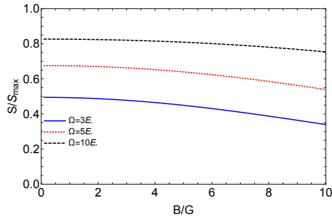
Fig. 4 The relative entanglement entropy, S/S_{\max} , as a function of the external magnetic field at different Raman coupling strength \Omega = 3, 5, 10 E_r using the scheme of Ref. 17 . All Raman laser detunings are zero.
